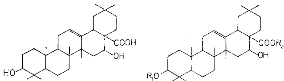
Acid echinocystic
