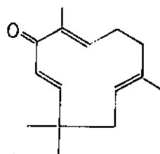
Zerumbone
