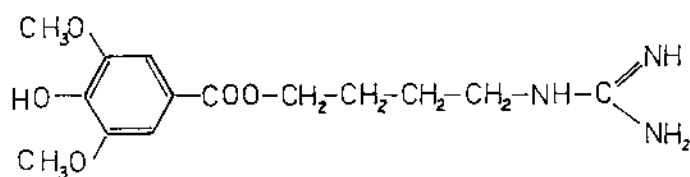
Leonurin
